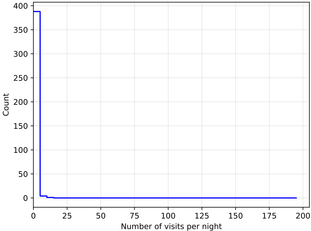
noroll_v3.4_10yrs all bands: DD:WFD NVisitsPerNight
