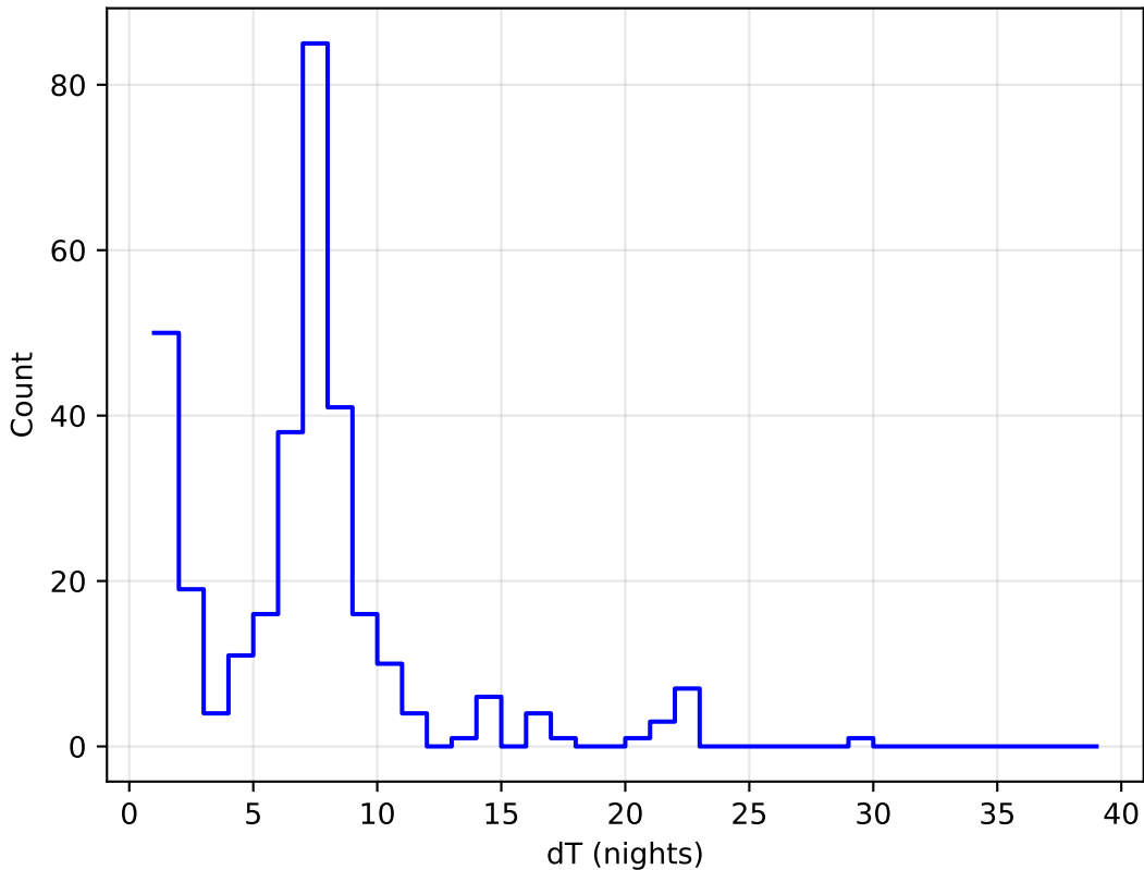
noroll_v3.4_10yrs all bands: DD:EDFS Delta Nights Histogram
