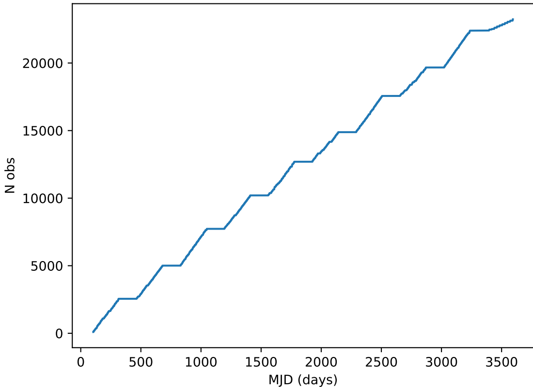
noroll_v3.4_10yrs all bands: DD:EDFS Cumulative NVisits
