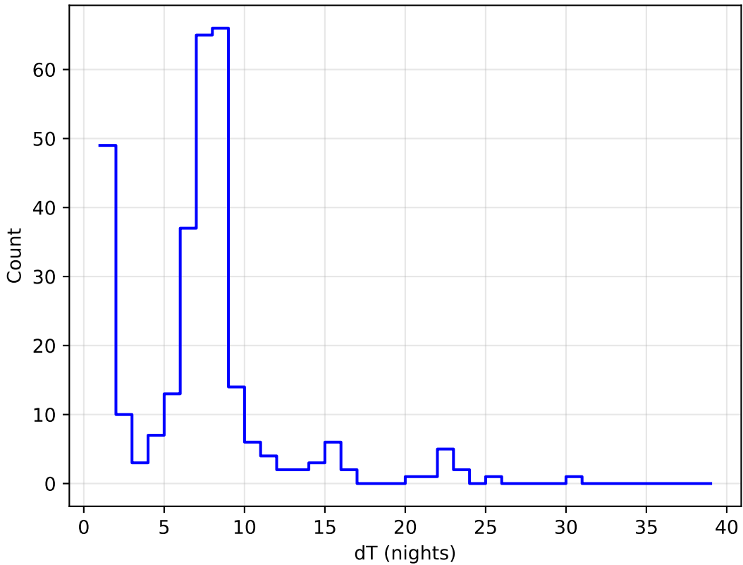
noroll_v3.4_10yrs all bands: DD:ECDFS Delta Nights Histogram
