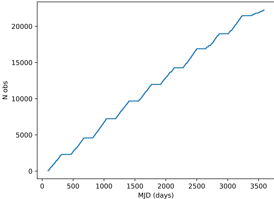
noroll_v3.4_10yrs all bands: DD:ECDFS Cumulative NVisits
