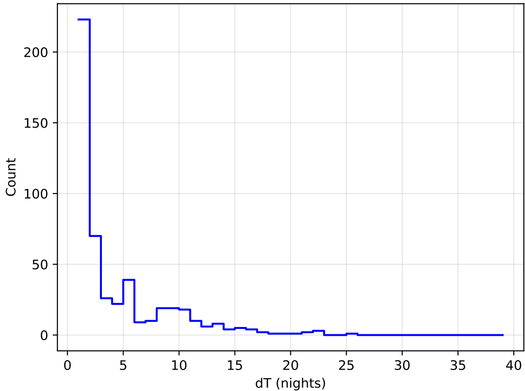
noroll_v3.4_10yrs all bands: DD: COSMOS Delta Nights Histogram
