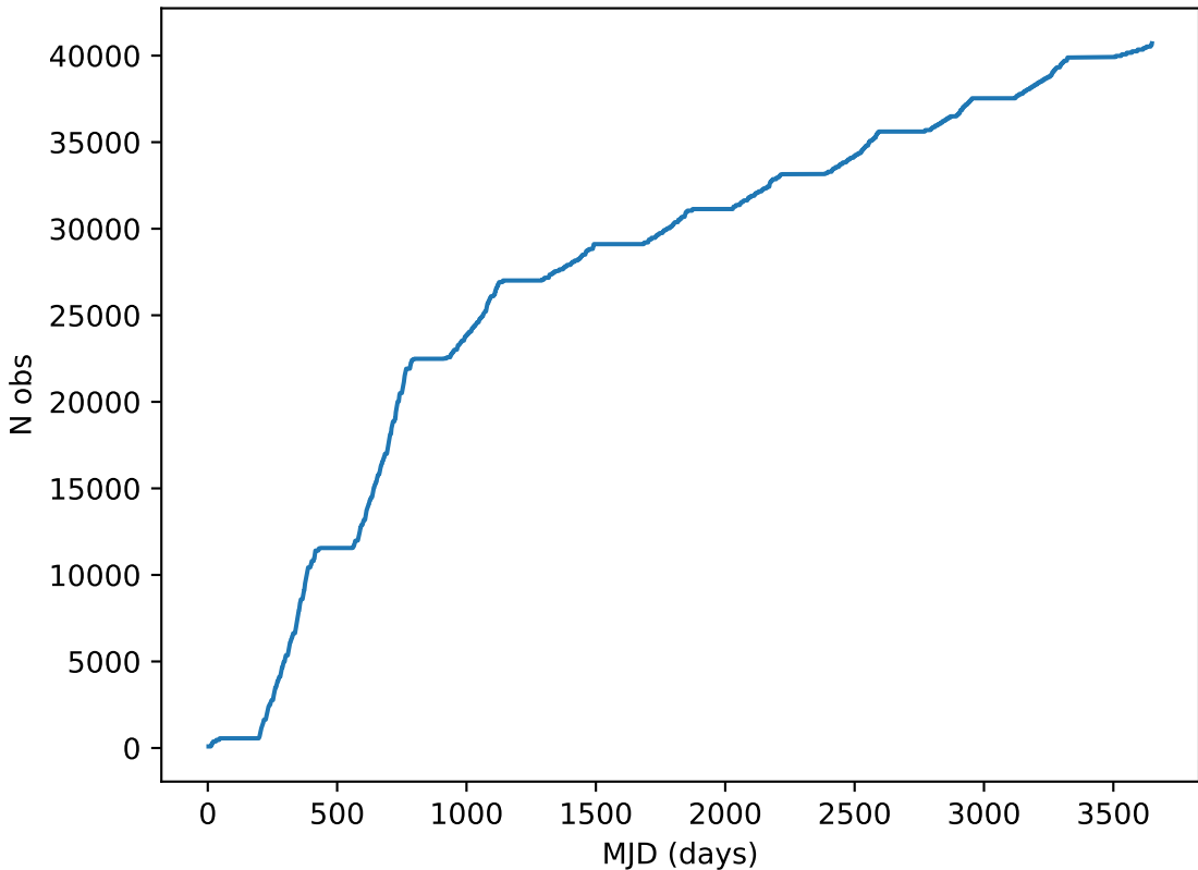
noroll_v3.4_10yrs all bands: DD: COSMOS Cumulative NVisits
