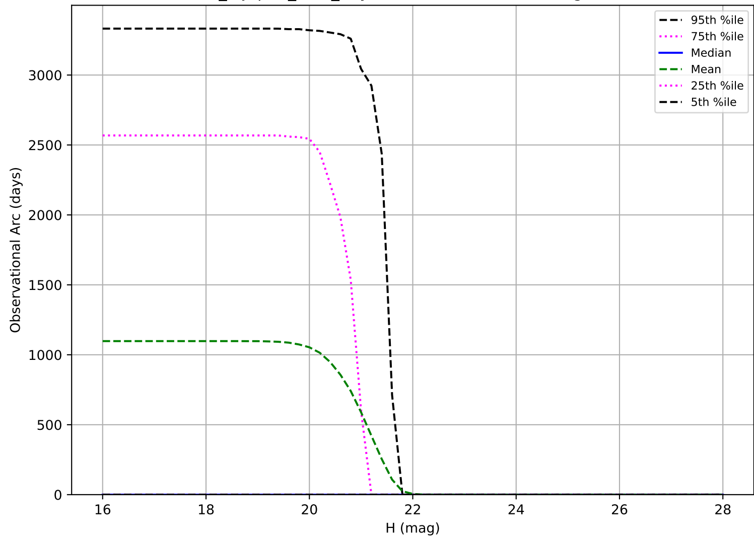
noroll_mjdp60_v3.4_10yrs: Observational Arc Length Vatira
