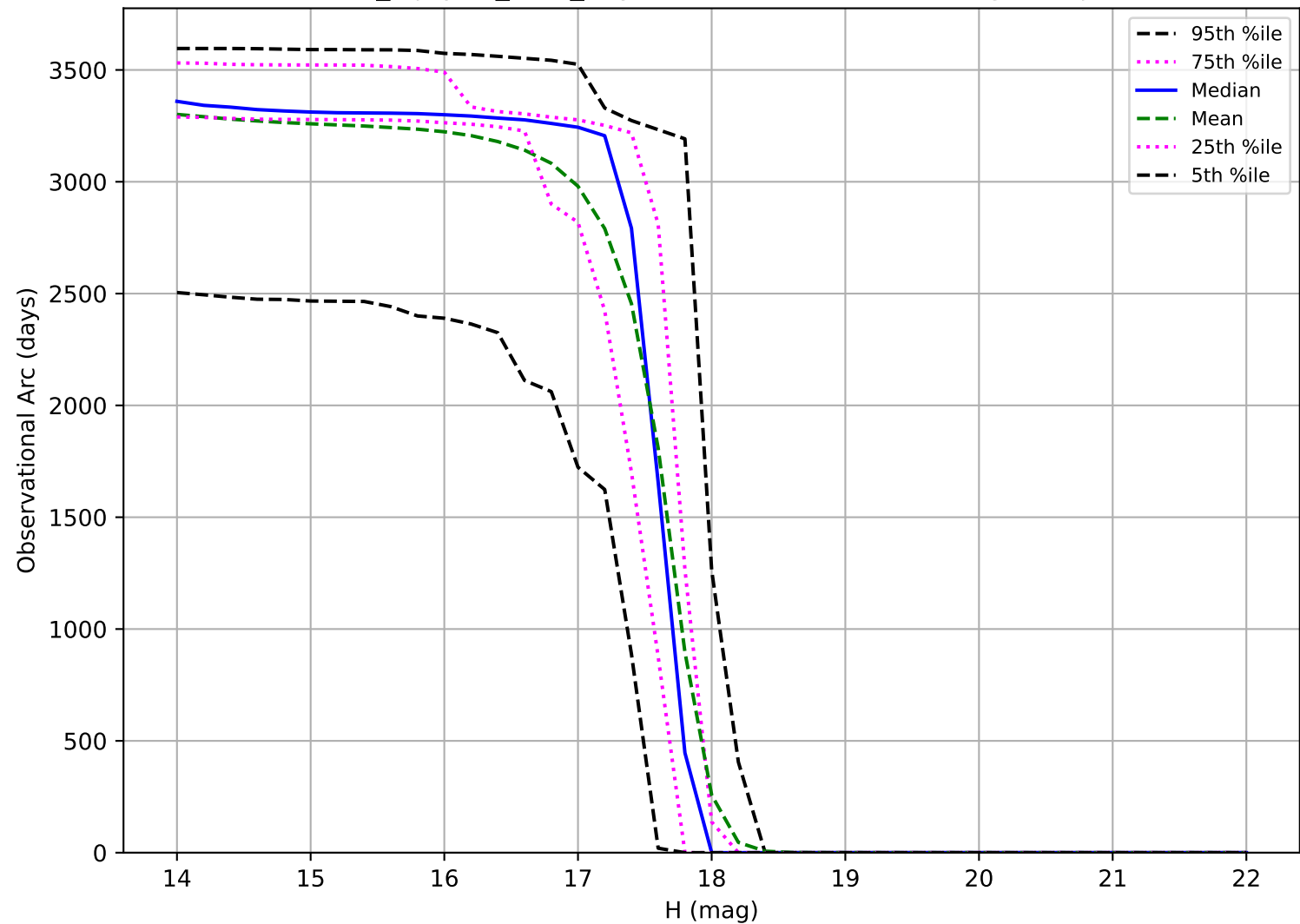
noroll_mjdp60_v3.4_10yrs: Observational Arc Length Trojan
