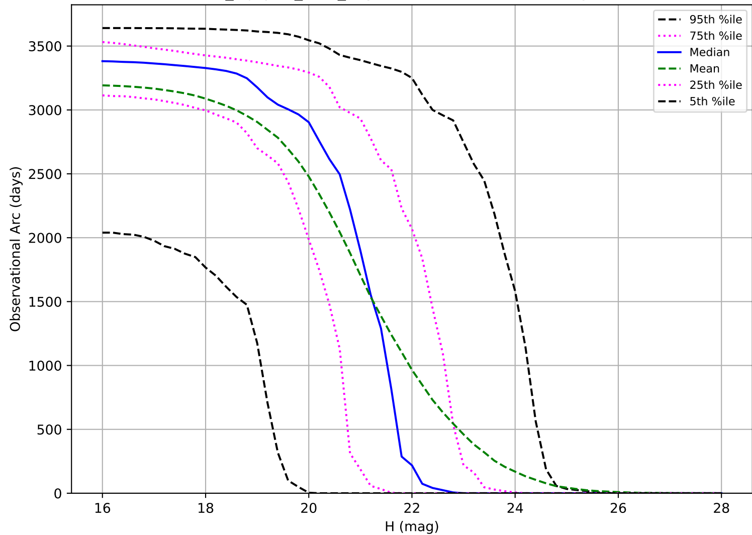
noroll_mjdp60_v3.4_10yrs: Observational Arc Length PHA
