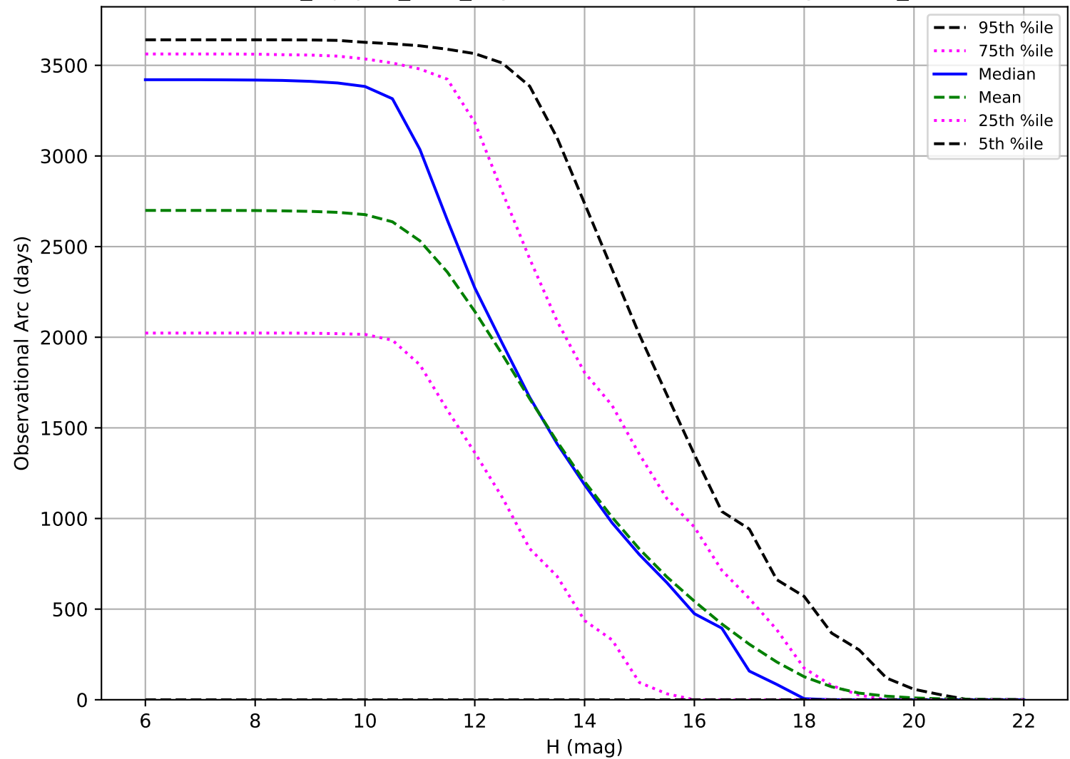
noroll_mjdp60_v3.4_10yrs: Observational Arc Length OCC_r5
