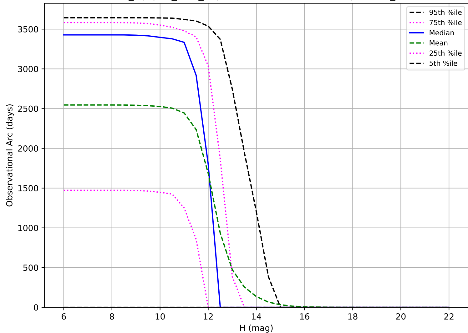
noroll_mjdp60_v3.4_10yrs: Observational Arc Length OCC_r20
