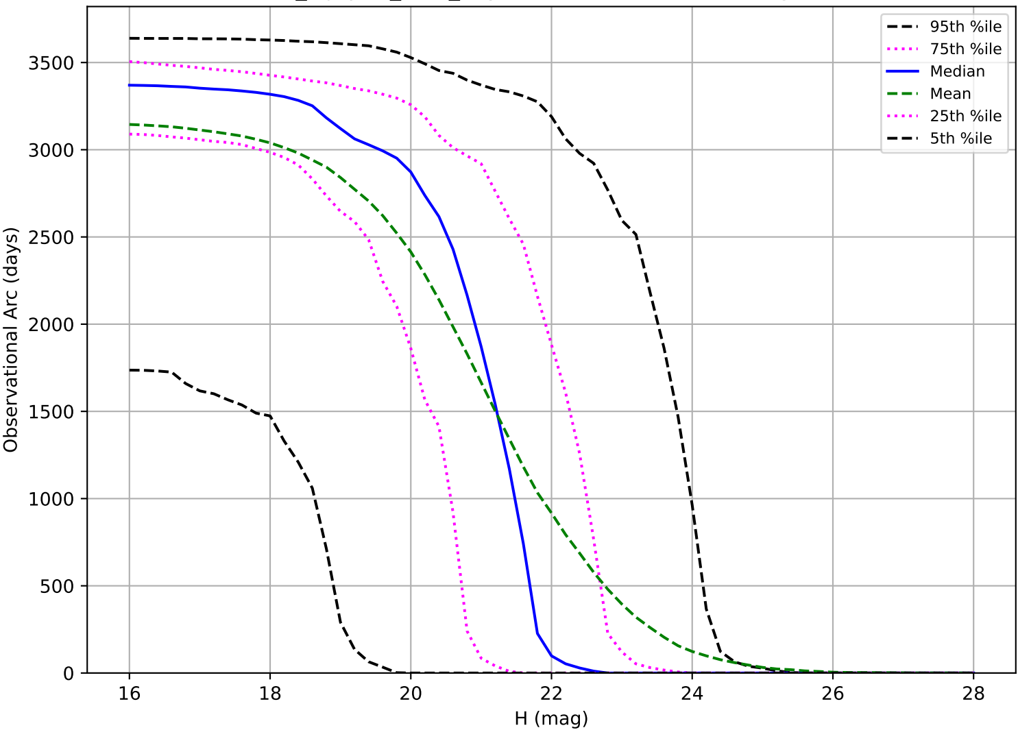
noroll_mjdp60_v3.4_10yrs: Observational Arc Length NEO
