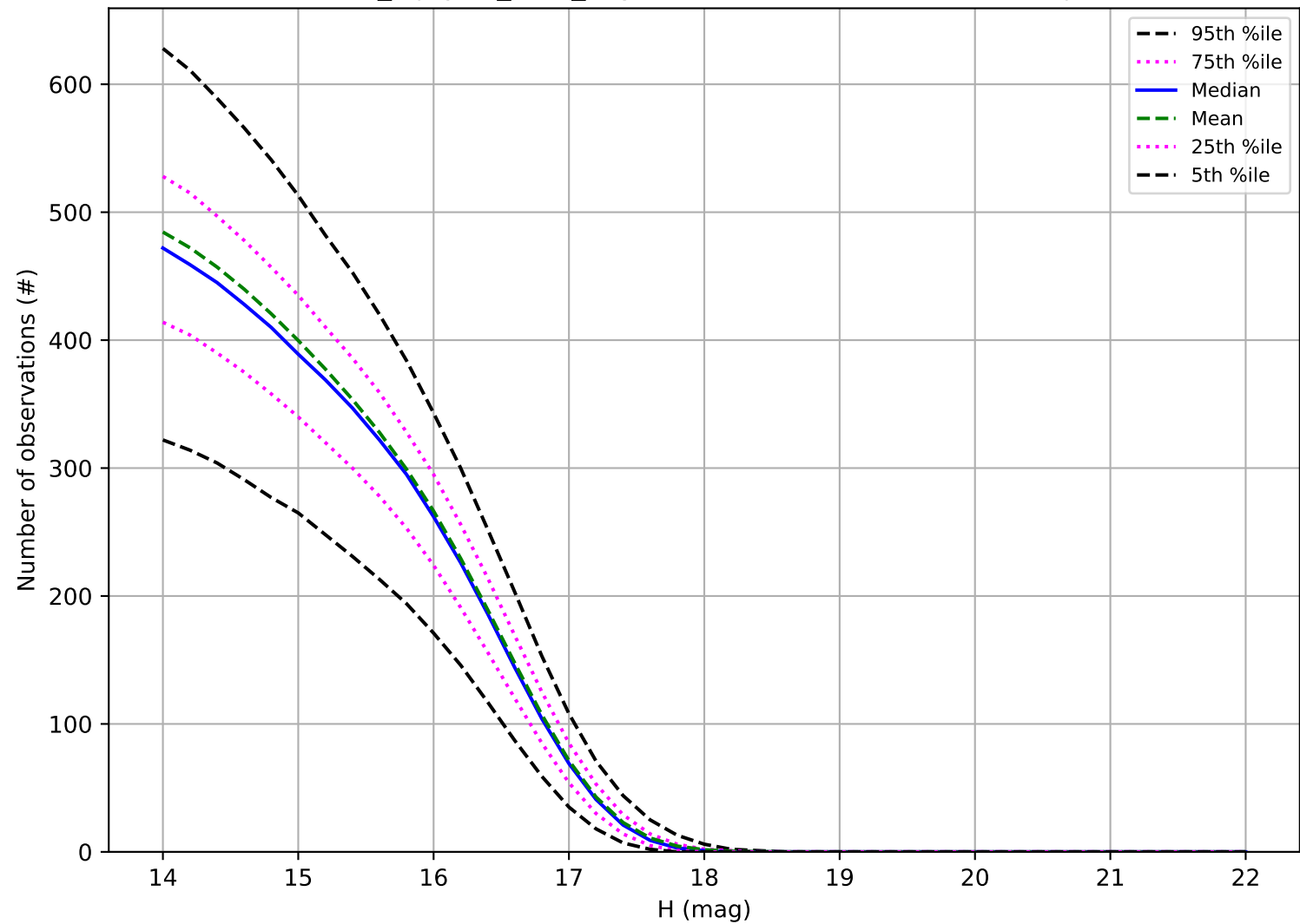
noroll_mjdp60_v3.4_10yrs: Number of observations Trojan
