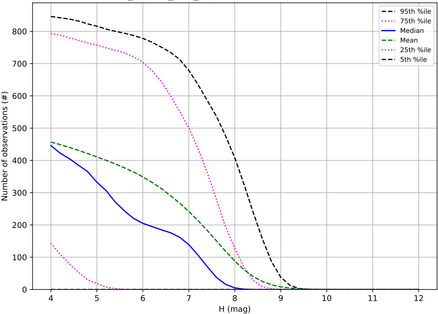
noroll_mjdp60_v3.4_10yrs: Number of observations TNO
