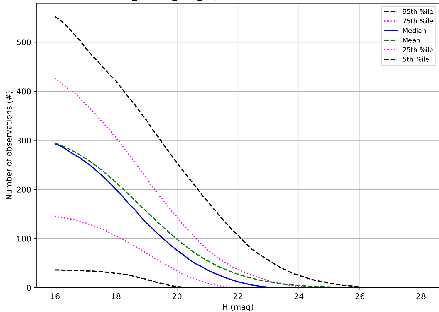
noroll_mjdp60_v3.4_10yrs: Number of observations PHA
