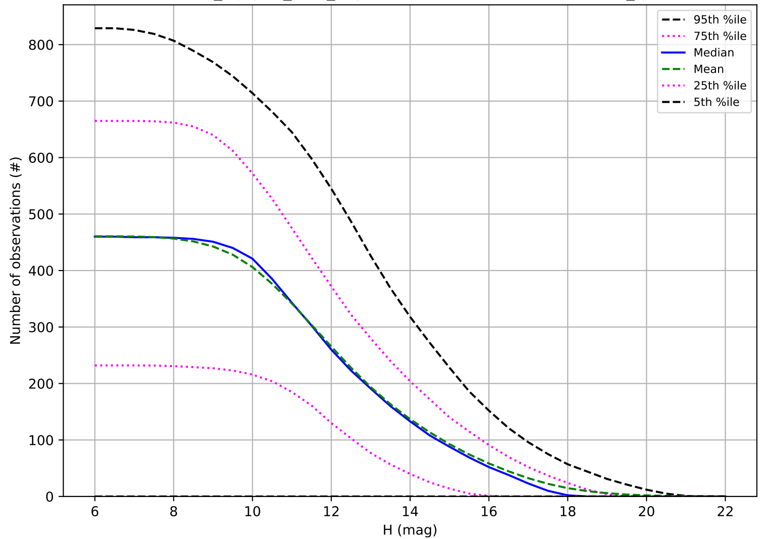
noroll_mjdp60_v3.4_10yrs: Number of observations OCC_r5
