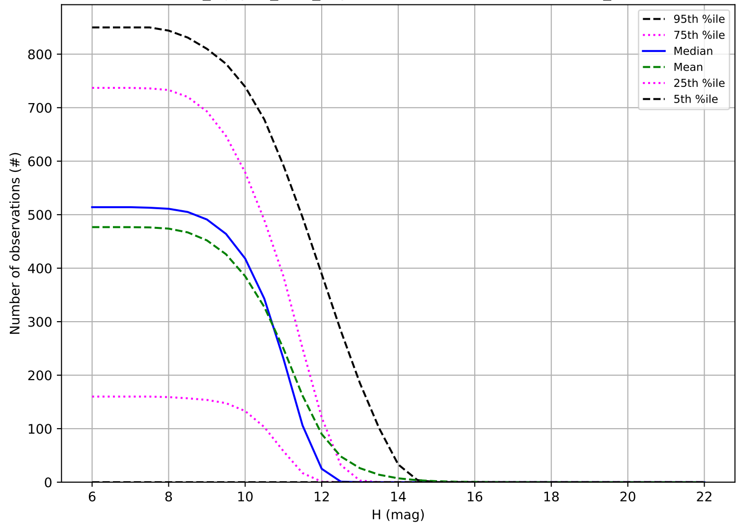
noroll_mjdp60_v3.4_10yrs: Number of observations OCC_r20
