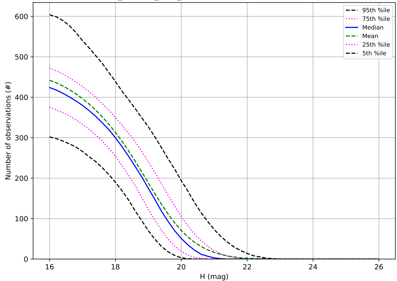
noroll_mjdp60_v3.4_10yrs: Number of observations MBA
