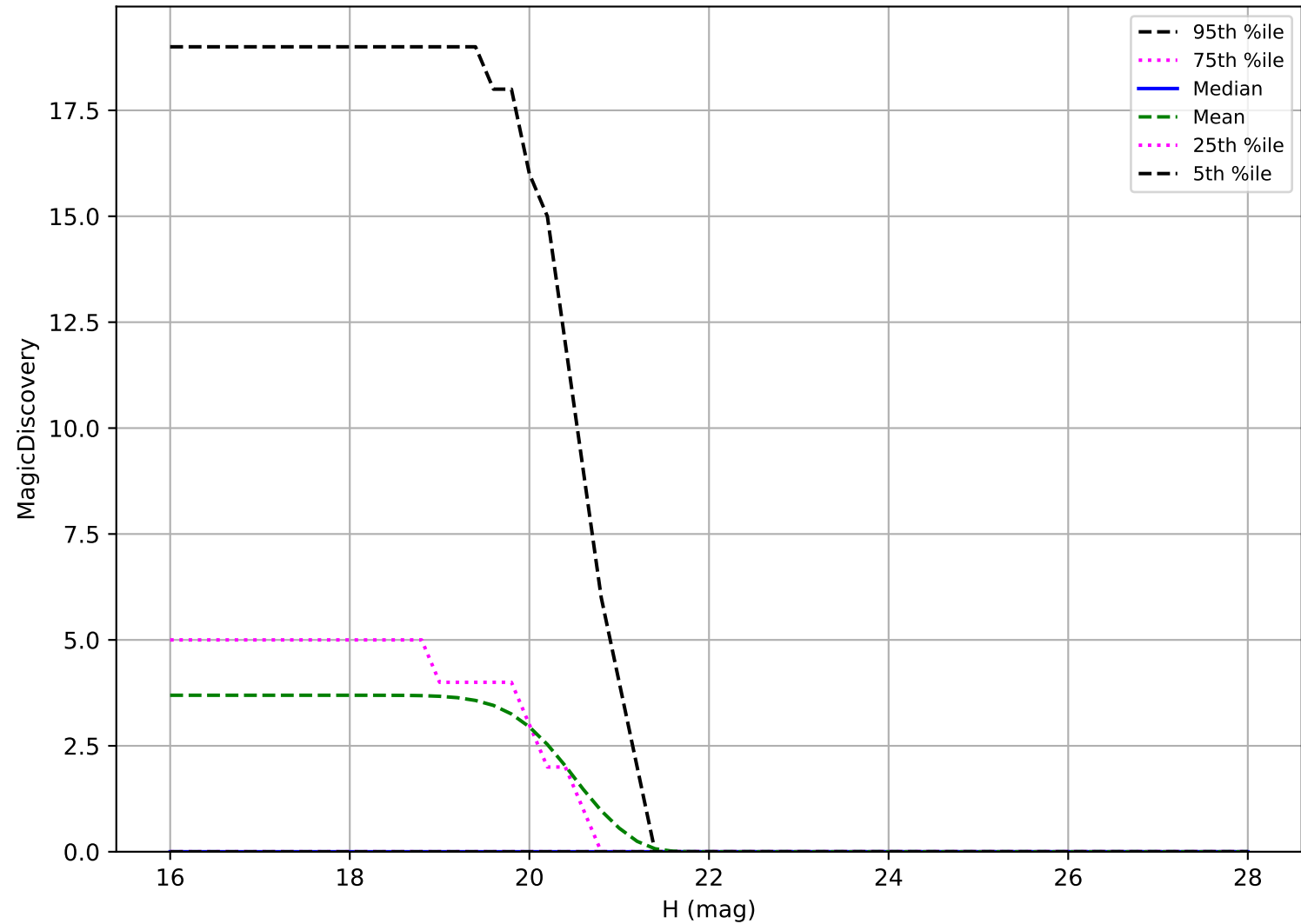
noroll_mjdp60_v3.4_10yrs: Vatira 6 detections in 60 nights detection loss
