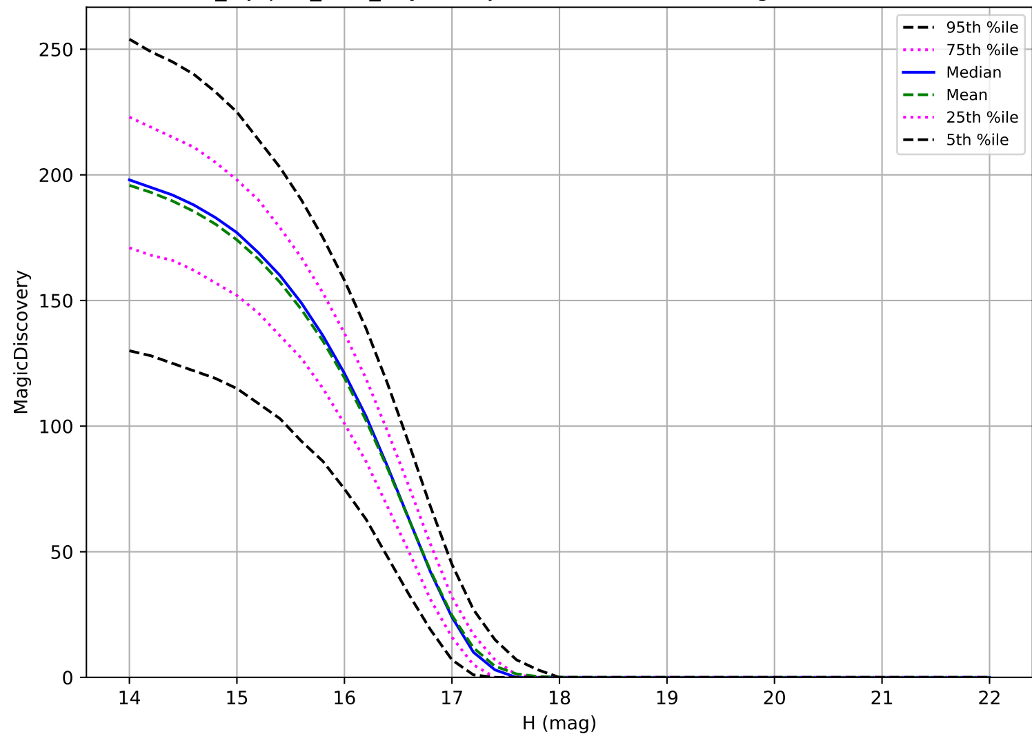
noroll_mjdp60_v3.4_10yrs: Trojan 6 detections in 60 nights detection loss
