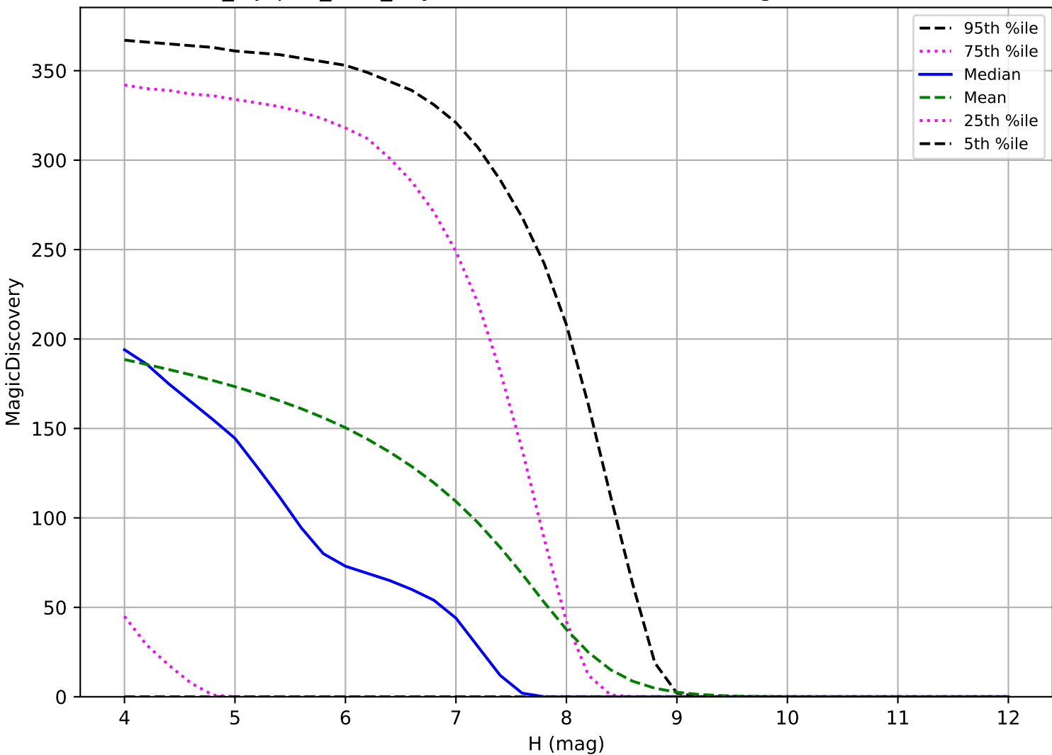
noroll_mjdp60_v3.4_10yrs: TNO 6 detections in 60 nights detection loss
