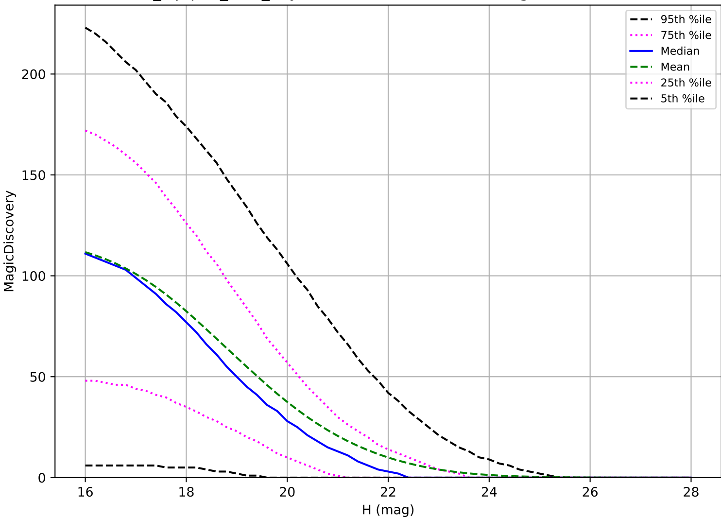
noroll_mjdp60_v3.4_10yrs: PHA 6 detections in 60 nights detection loss
