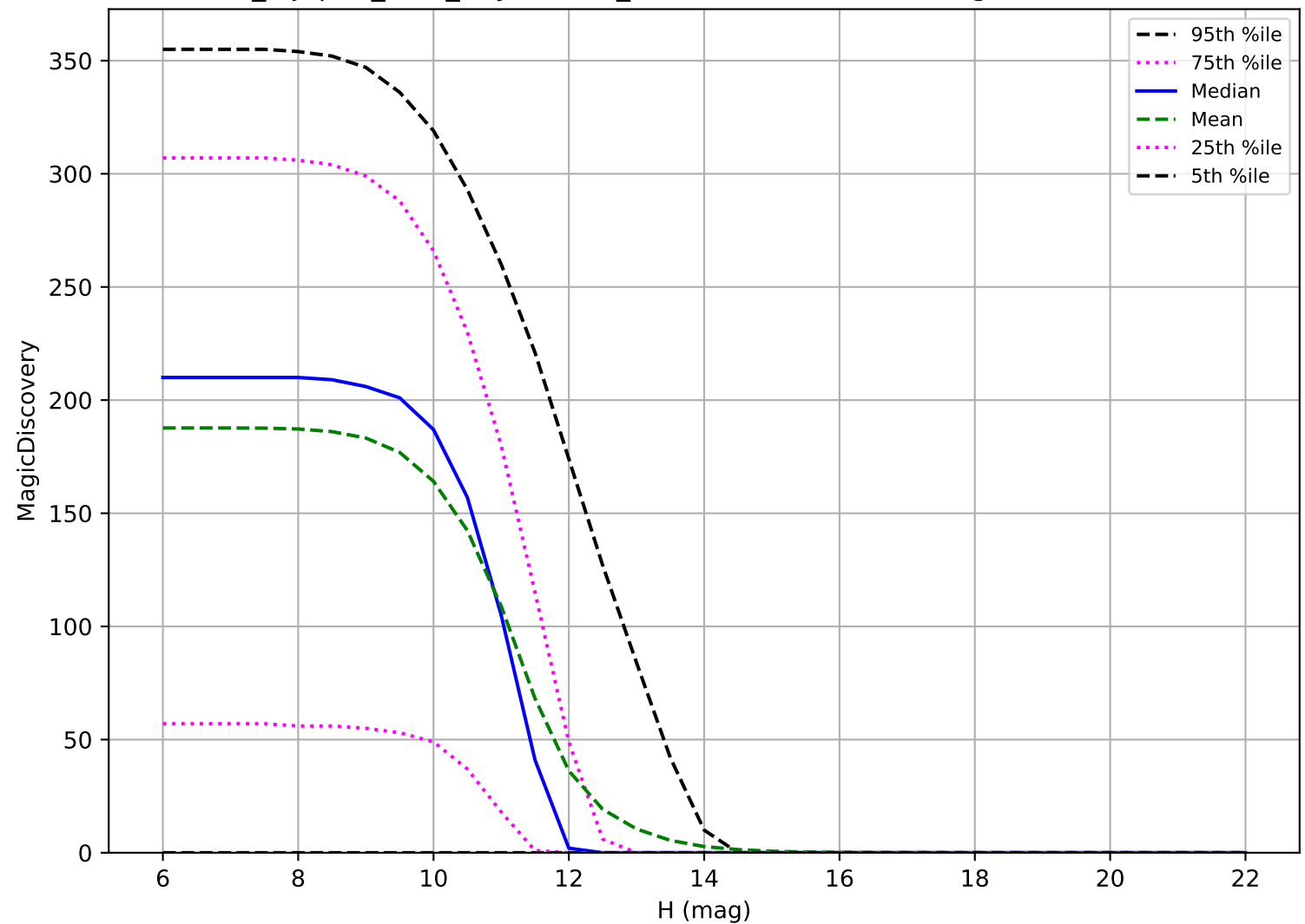
noroll_mjdp60_v3.4_10yrs: OCC_r20 6 detections in 60 nights detection loss
