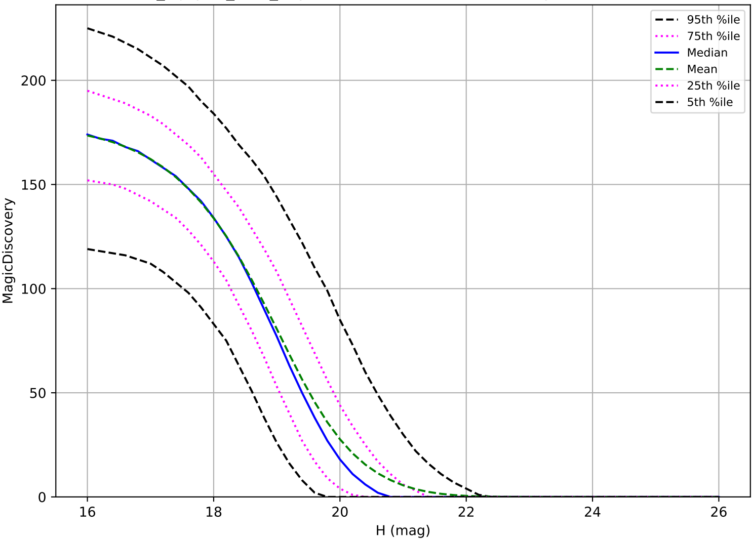
noroll_mjdp60_v3.4_10yrs: MBA 6 detections in 60 nights detection loss
