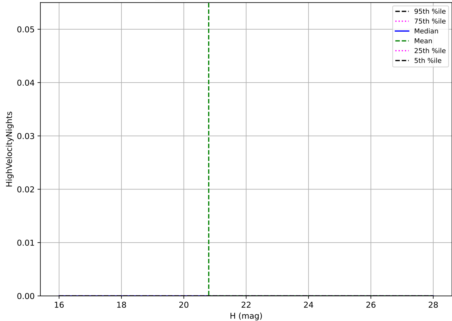
noroll_mjdp60_v3.4_10yrs: Vatira High velocity pair detection loss
