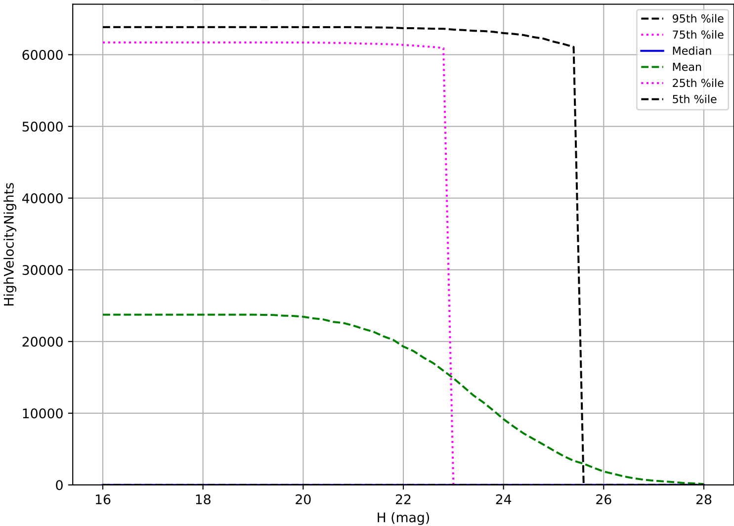
noroll_mjdp60_v3.4_10yrs: PHA High velocity pair detection loss
