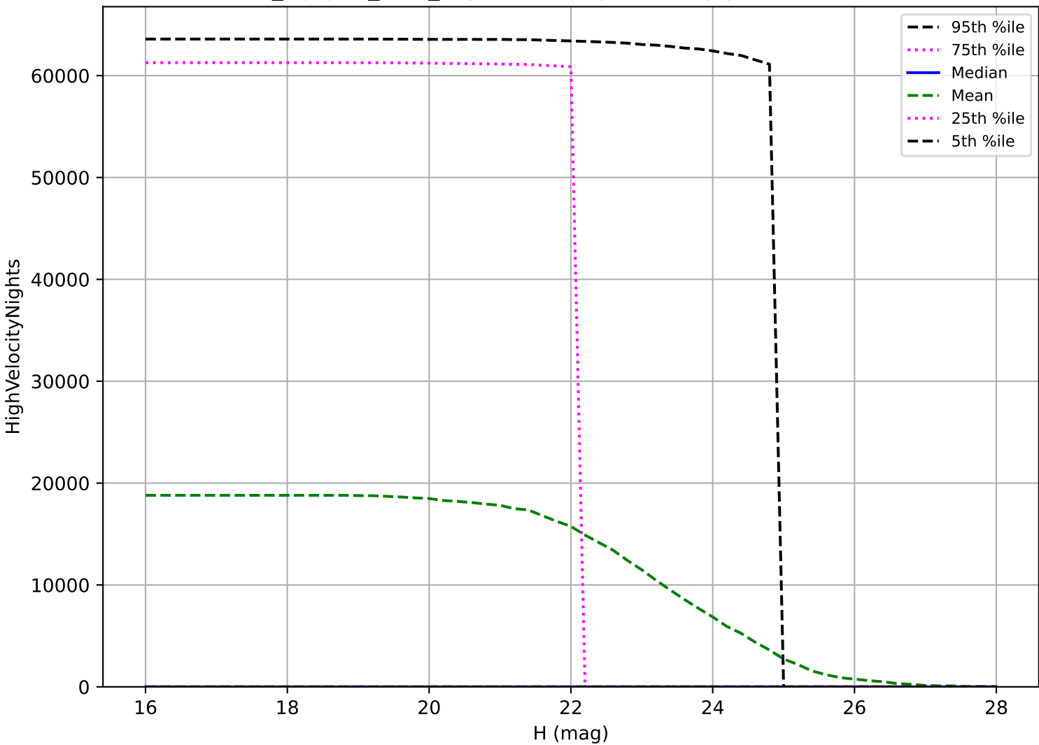
noroll_mjdp60_v3.4_10yrs: NEO High velocity pair detection loss
