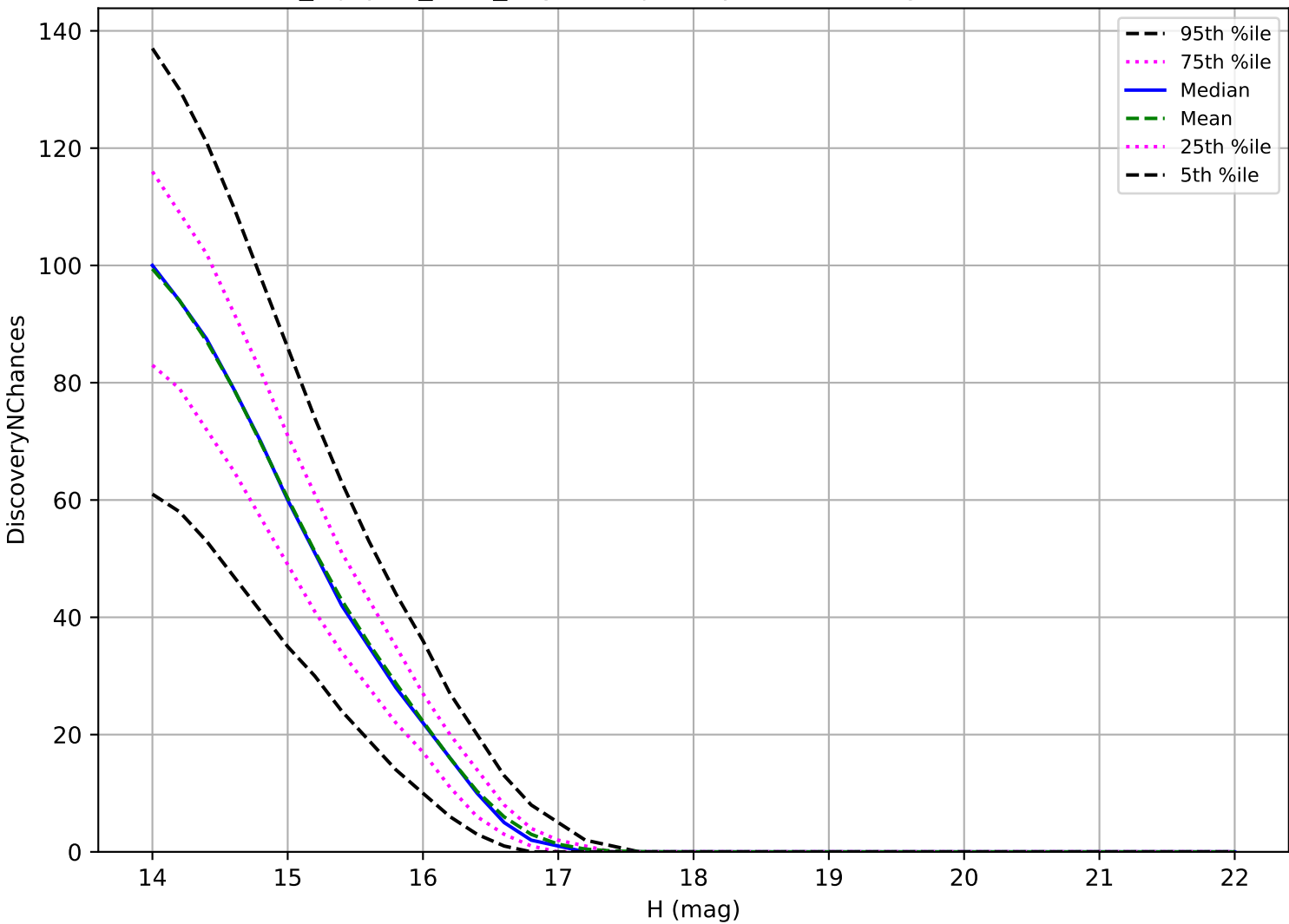
noroll_mjdp60_v3.4_10yrs: Trojan 3 pairs in 15 nights detection loss
