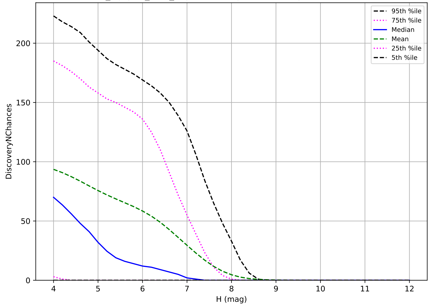
noroll_mjdp60_v3.4_10yrs: TNO 3 pairs in 15 nights detection loss
