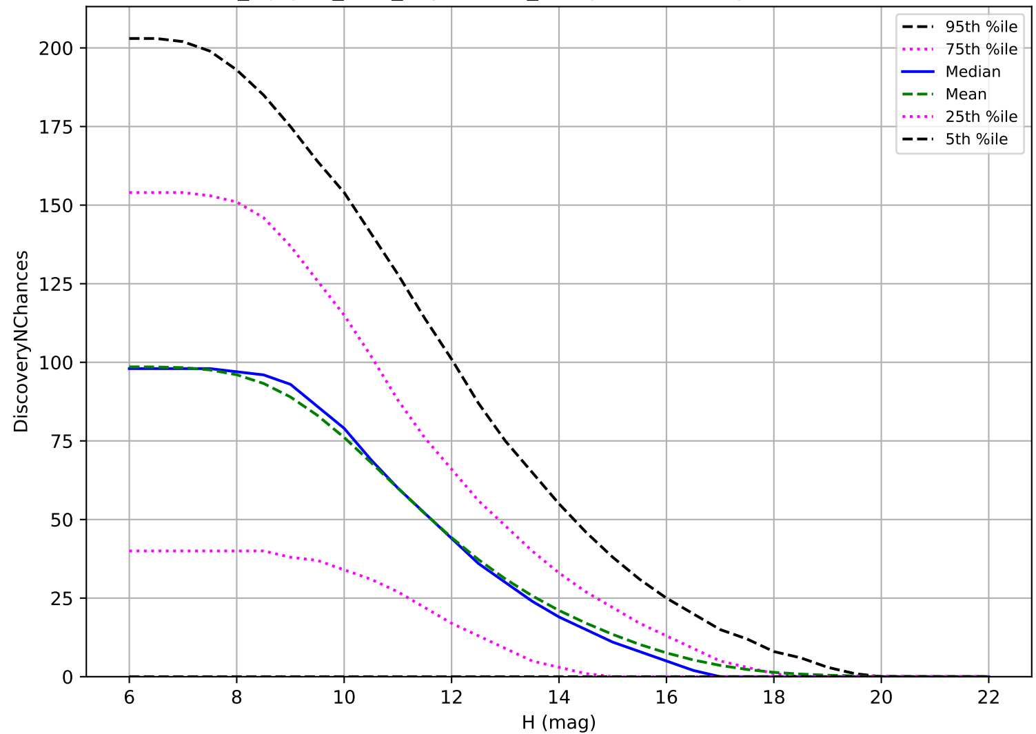
noroll_mjdp60_v3.4_10yrs: OCC_r5 3 pairs in 15 nights detection loss
