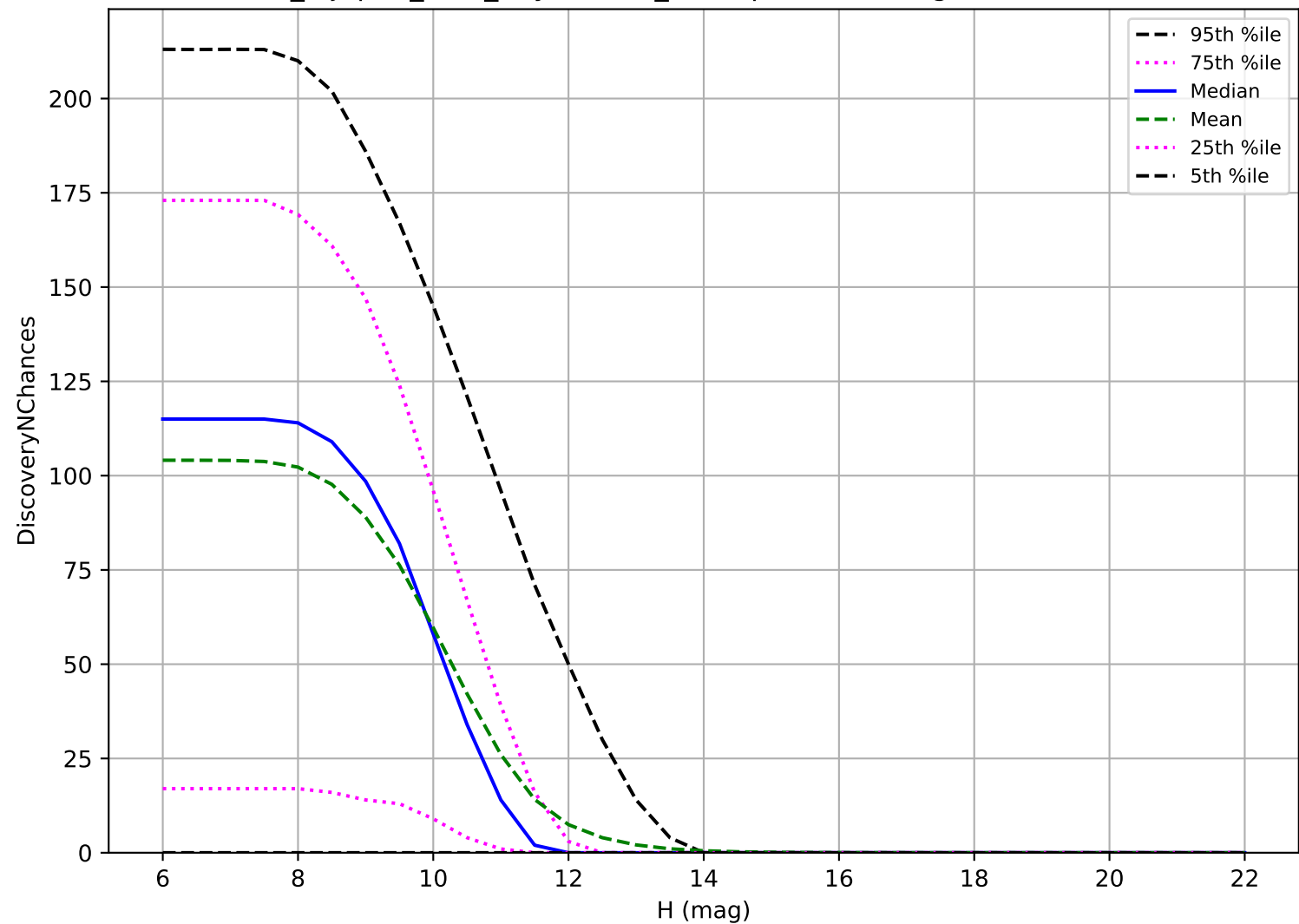
noroll_mjdp60_v3.4_10yrs: OCC_r20 3 pairs in 15 nights detection loss
