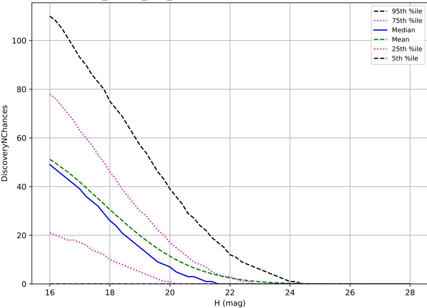
noroll_mjdp60_v3.4_10yrs: NEO 3 pairs in 15 nights detection loss
