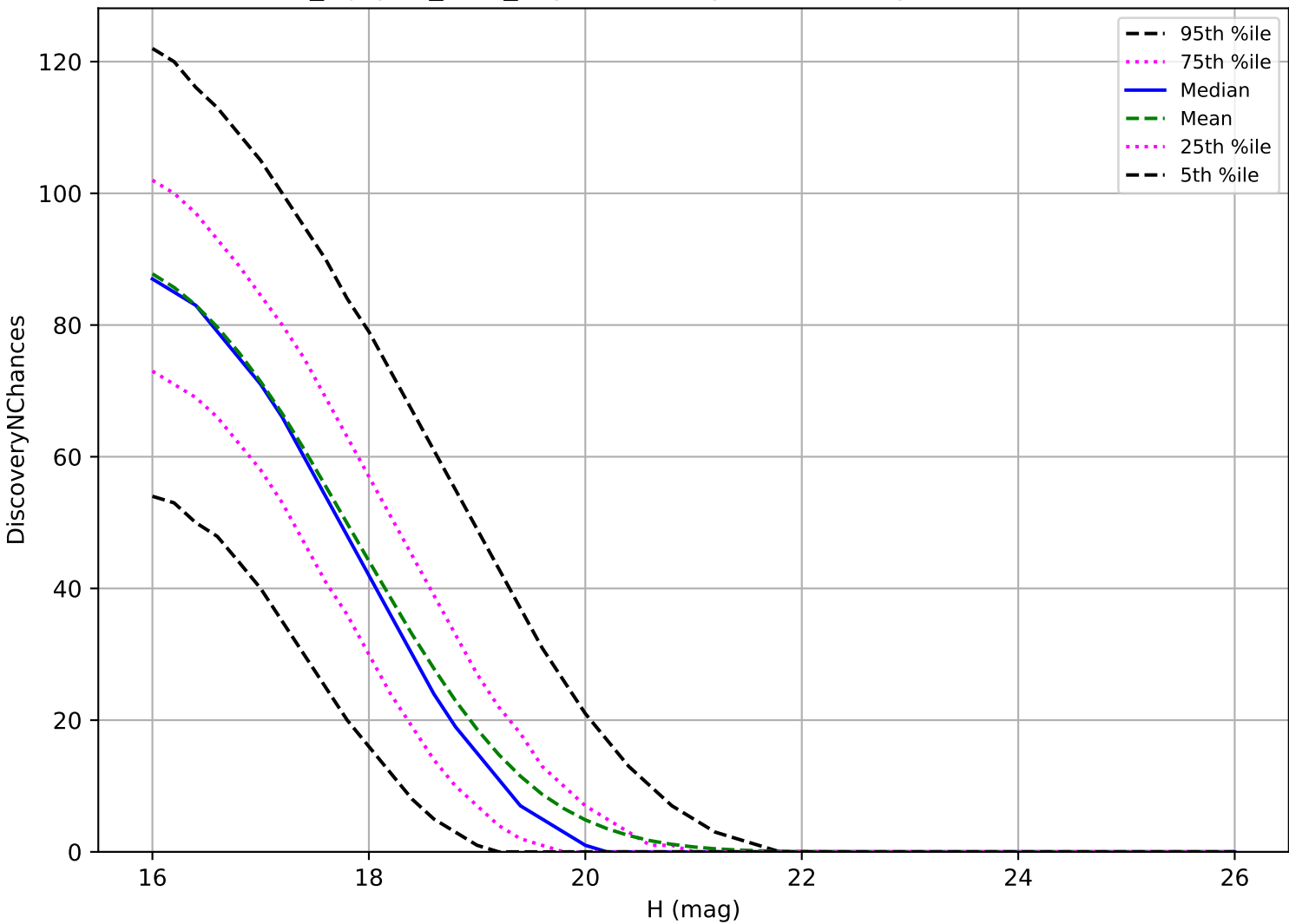
noroll_mjdp60_v3.4_10yrs: MBA 3 pairs in 15 nights detection loss
