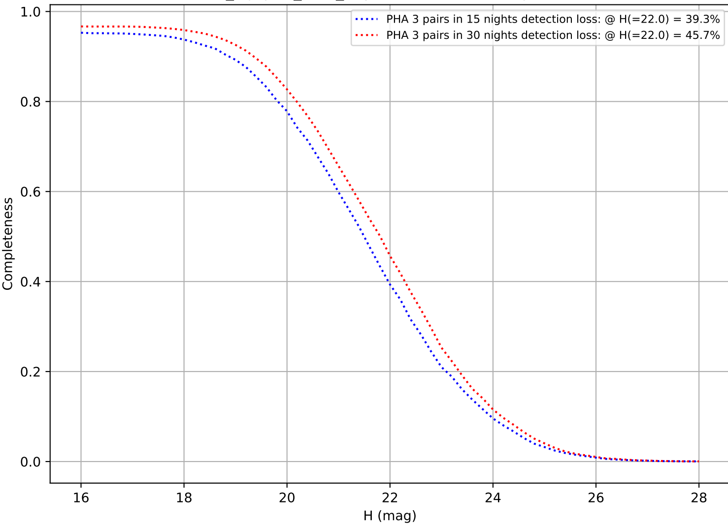
noroll_mjdp60_v3.4_10yrs: DifferentialCompleteness
