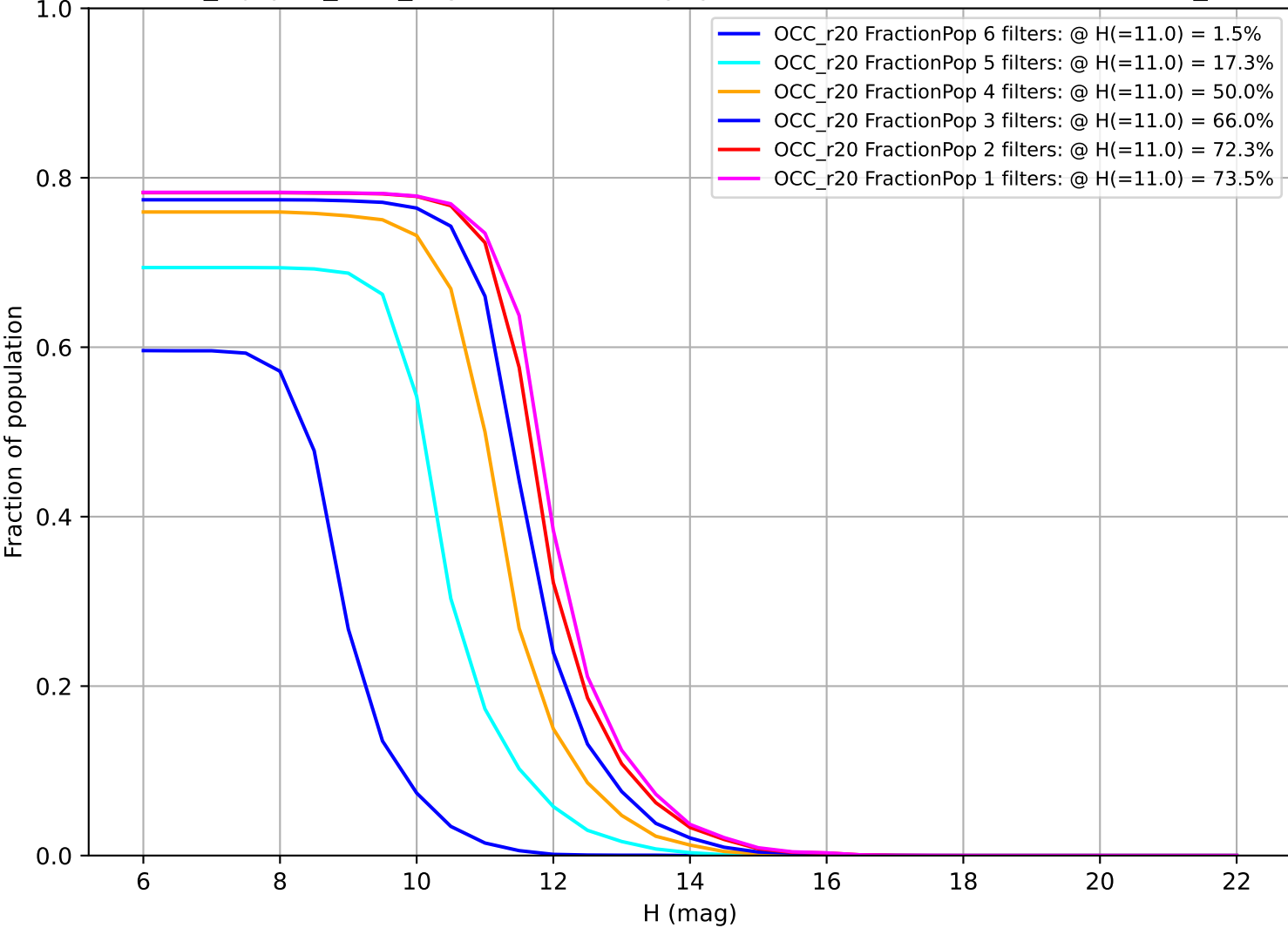
noroll_mjdp60_v3.4_10yrs: Fraction of population with colors in X filters OCC_r20
