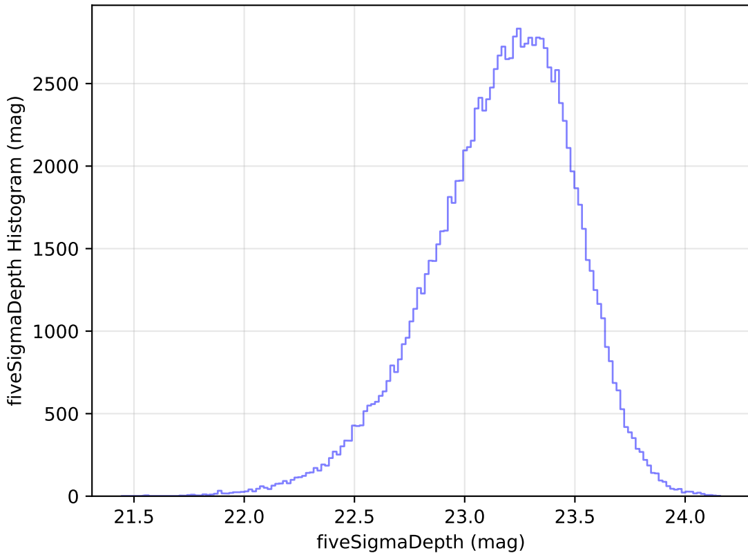
noroll_mjdp60_v3.4_10yrs u: fiveSigmaDepth Histogram
