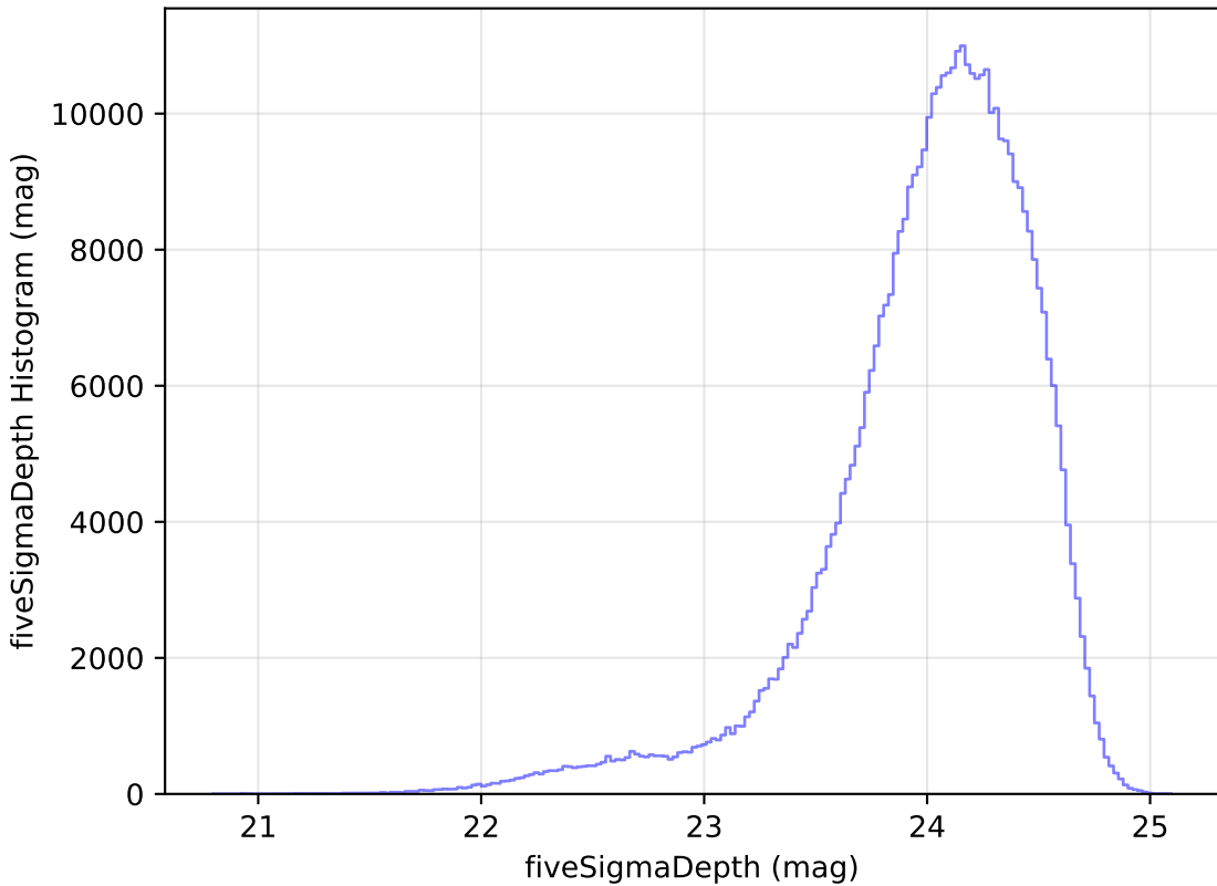
noroll_mjdp60_v3.4_10yrs r: fiveSigmaDepth Histogram
