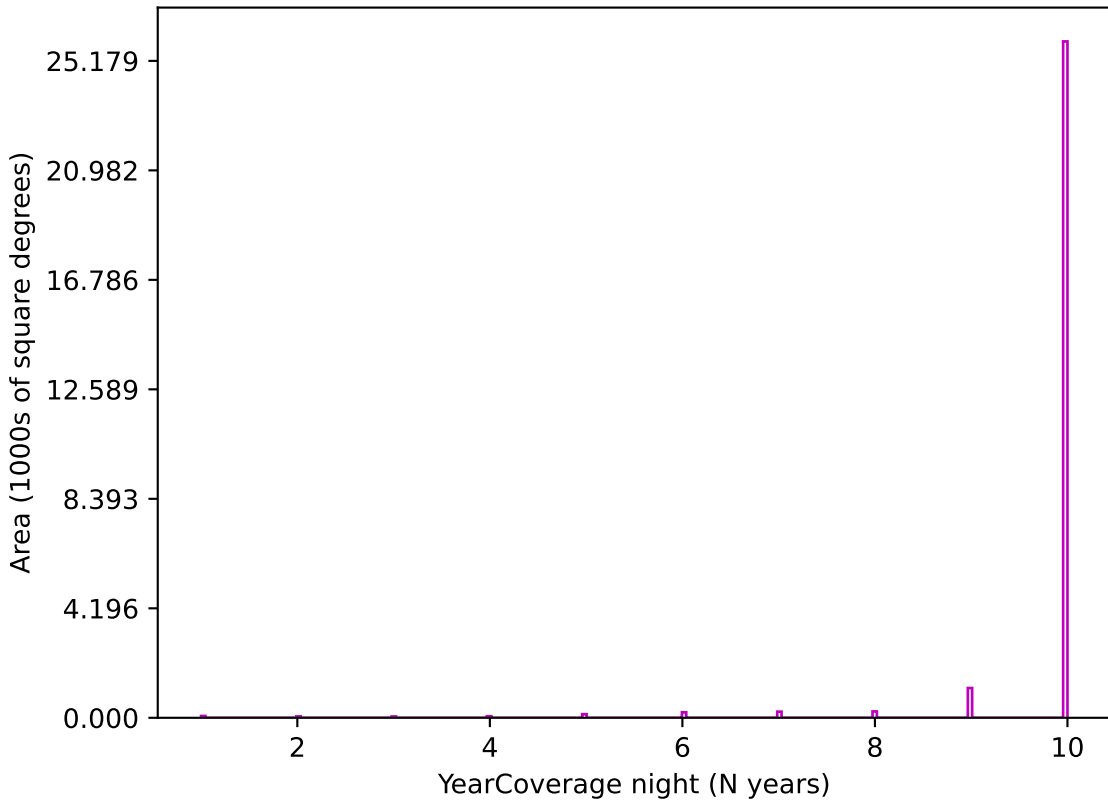
noroll_mjdp60_v3.4_10yrs z band: YearCoverage night
