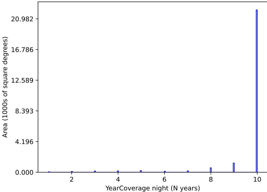
noroll_mjdp60_v3.4_10yrs y band: YearCoverage night
