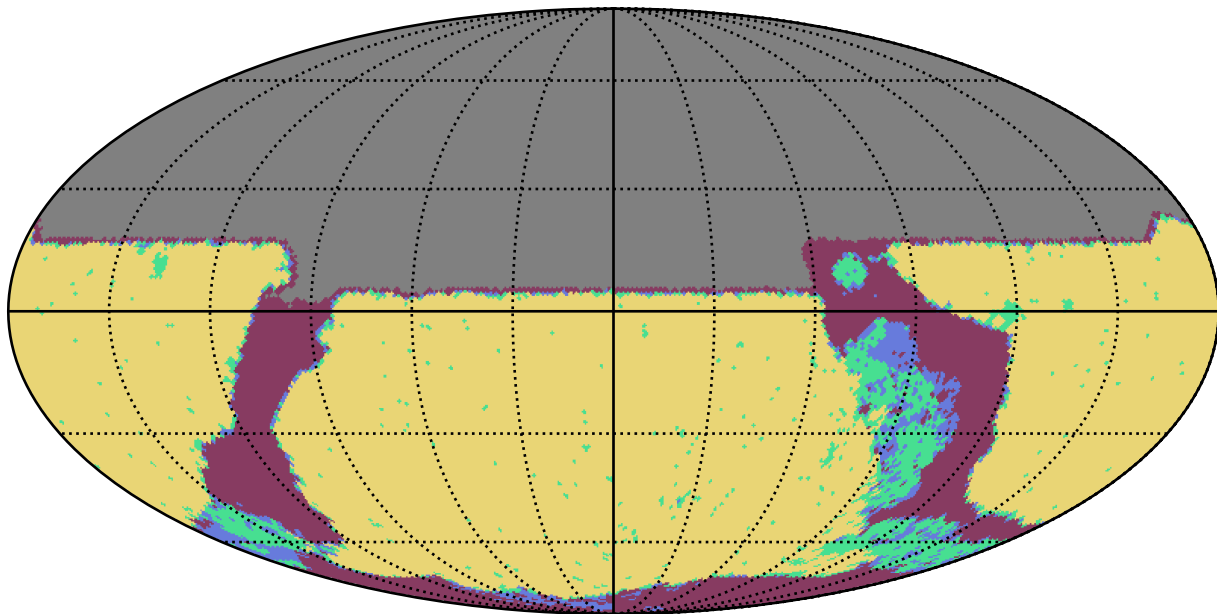
noroll_mjdp60_v3.4_10yrs u band: YearCoverage night
