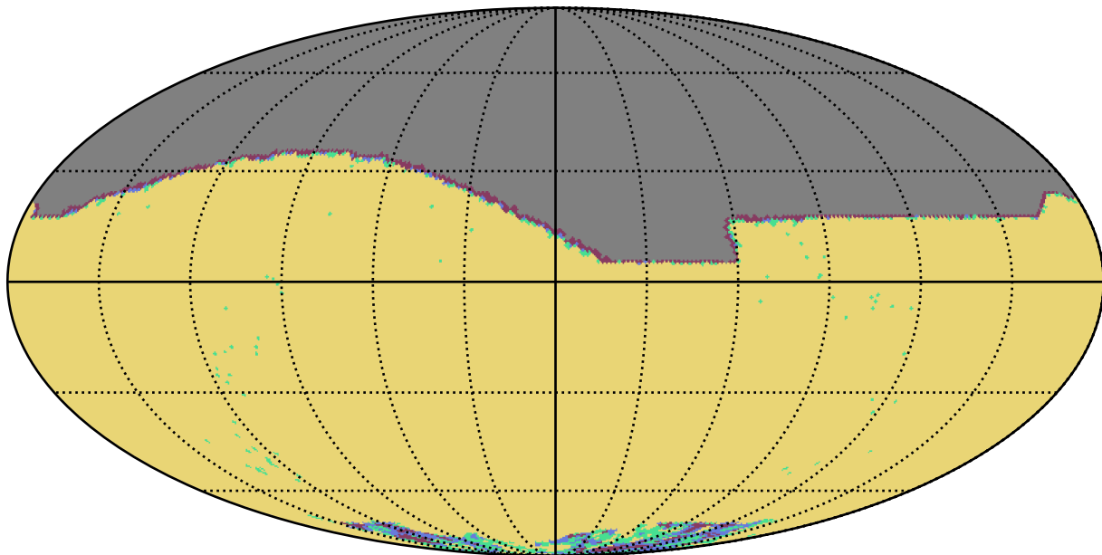
noroll_mjdp60_v3.4_10yrs i band: YearCoverage night
