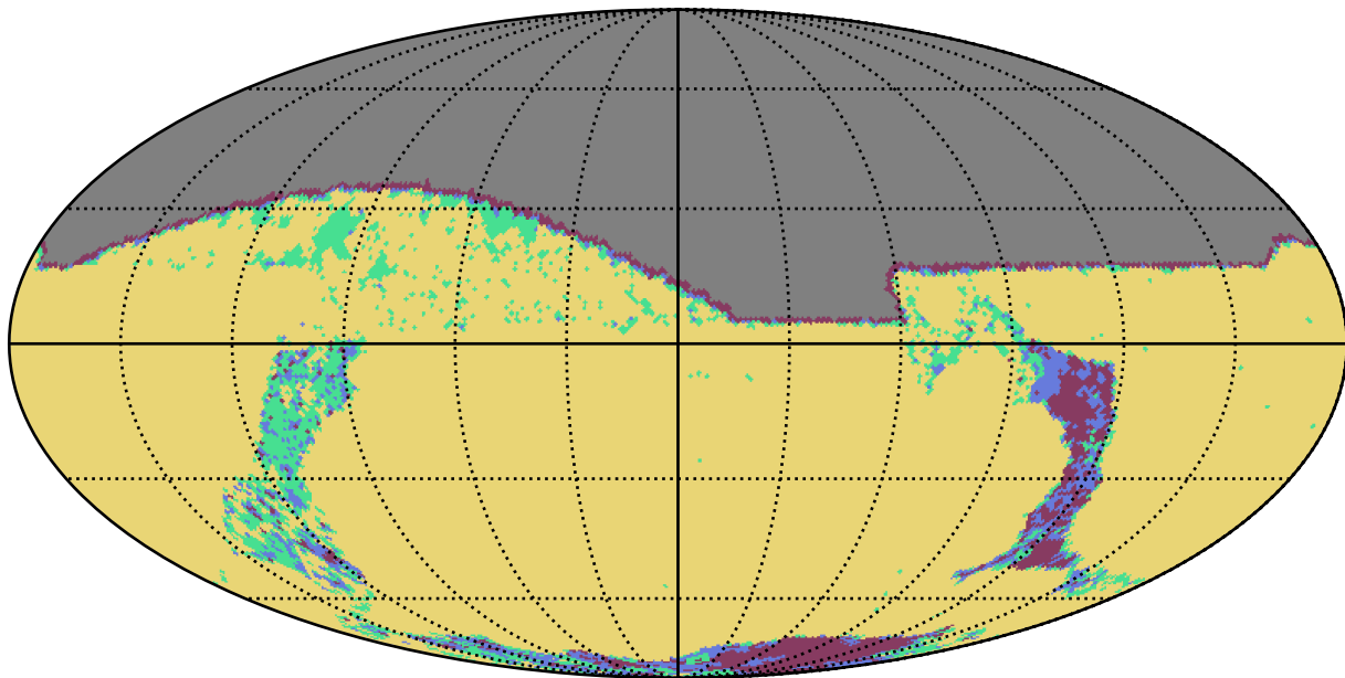
noroll_mjdp60_v3.4_10yrs g band: YearCoverage night
