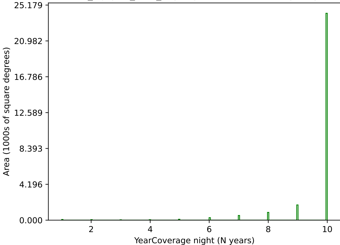
noroll_mjdp60_v3.4_10yrs g band: YearCoverage night
