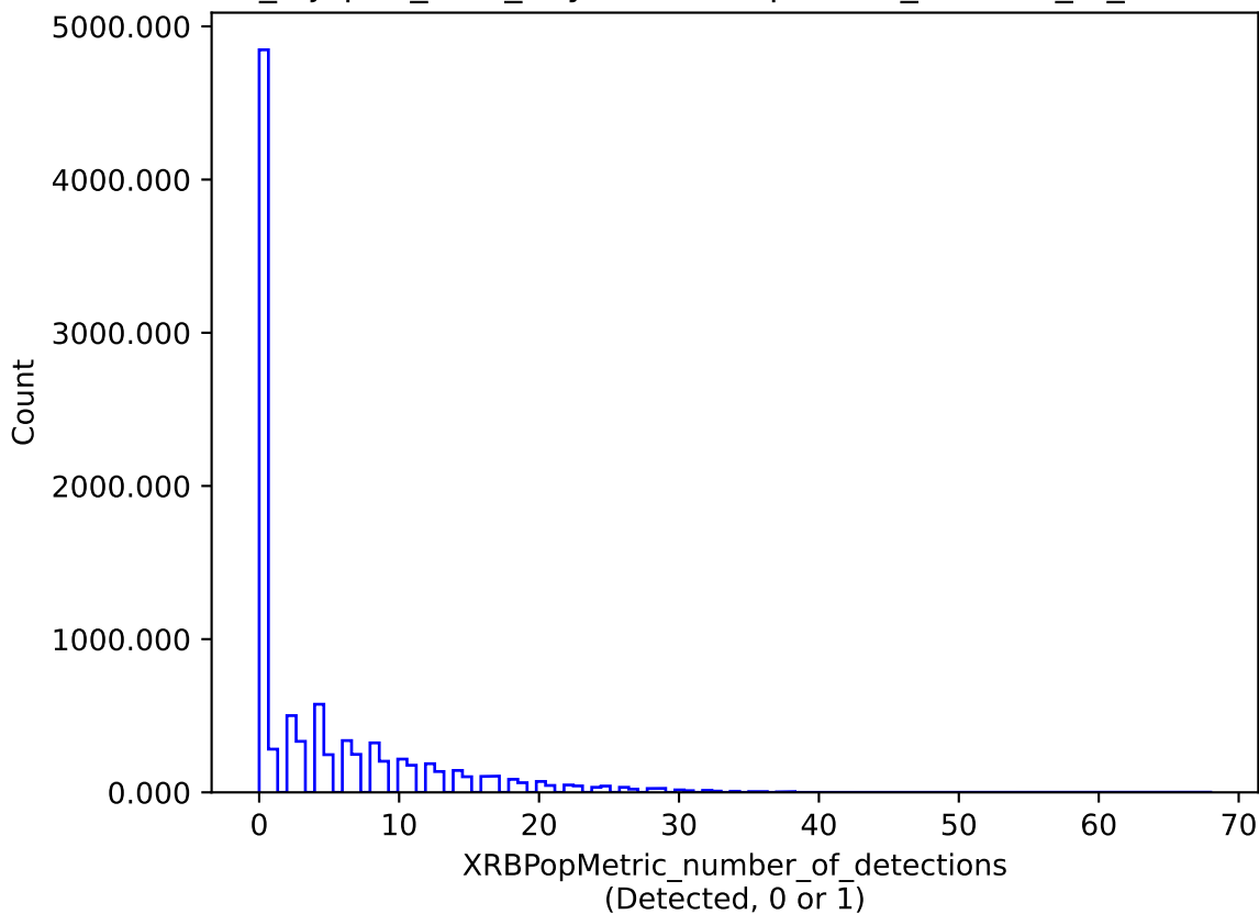
noroll_mjdp60_v3.4_10yrs : XRBPoMetric_number_of_detections
