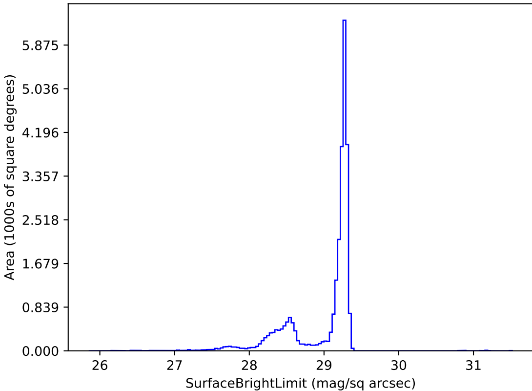
noroll_mjdp60_v3.4_10yrs z: SurfaceBrightLimit
