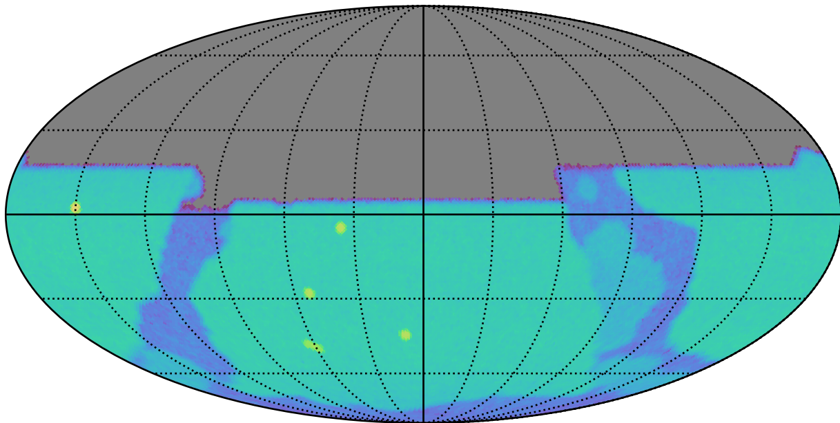
noroll_mjdp60_v3.4_10yrs u: SurfaceBrightLimit
