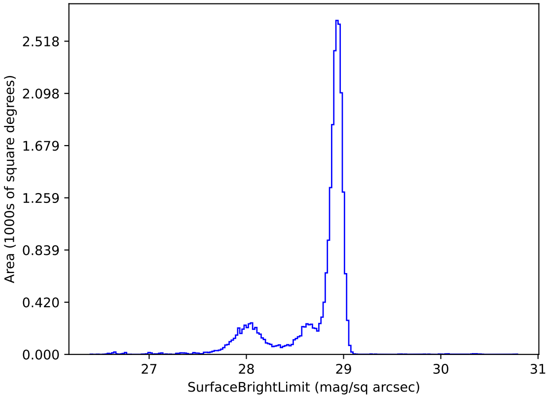
noroll_mjdp60_v3.4_10yrs u: SurfaceBrightLimit
