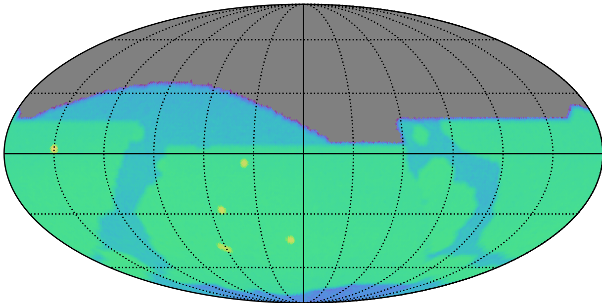
noroll_mjdp60_v3.4_10yrs r: SurfaceBrightLimit
