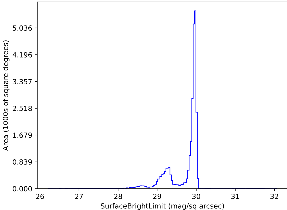
noroll_mjdp60_v3.4_10yrs i: SurfaceBrightLimit
